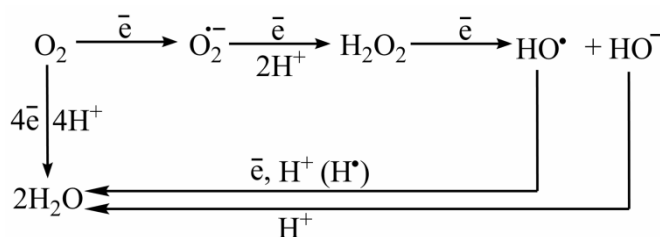
Fig. 1. Reduction of molecular oxygen via four- and one-electron schemes.
